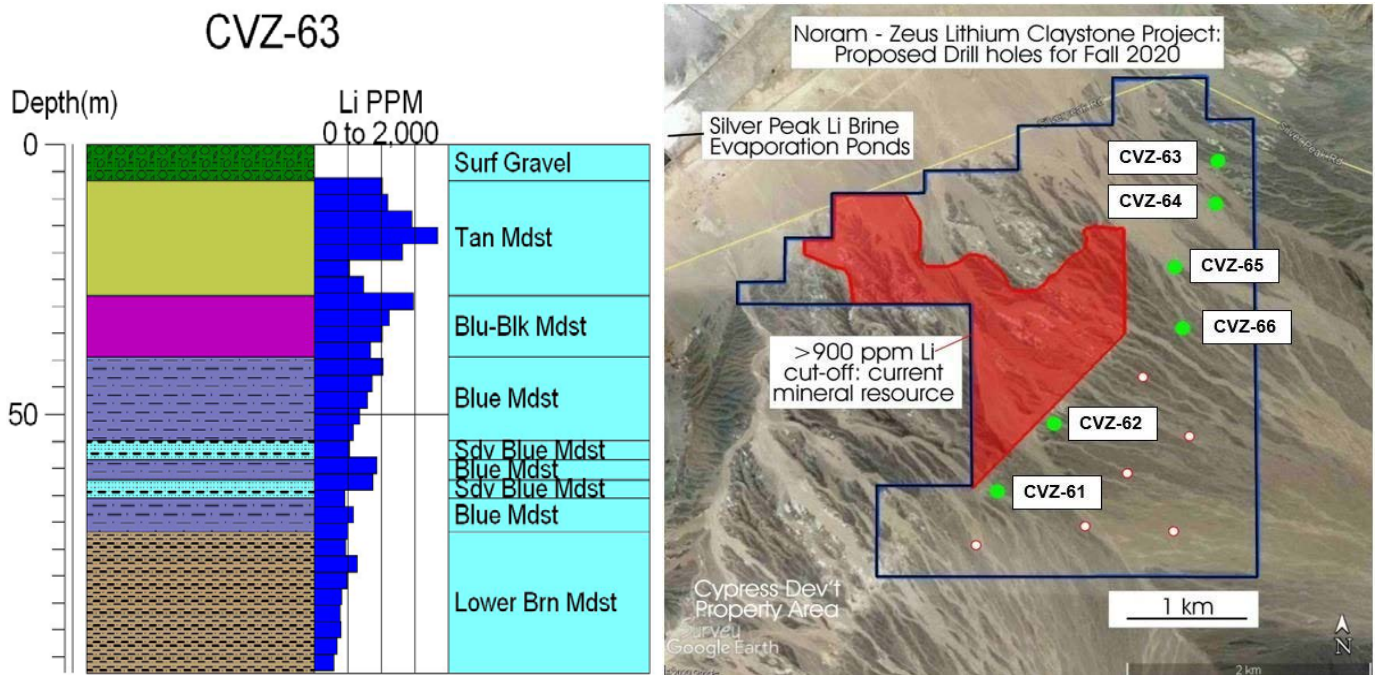
Figure 1a) Strip Log of CVZ-63 outlining the various claystone types encountered at depth from the surface to 322 ft (98.1m) b) Zeus Property map showing a) location of current Indicated and Inferred resources at >900ppm Li cut-off; b) location of drill sites completed or in progress (seen in green) to date for the Phase V 2020/2021 program. Proposed drill sites not yet explored indicated in white.
